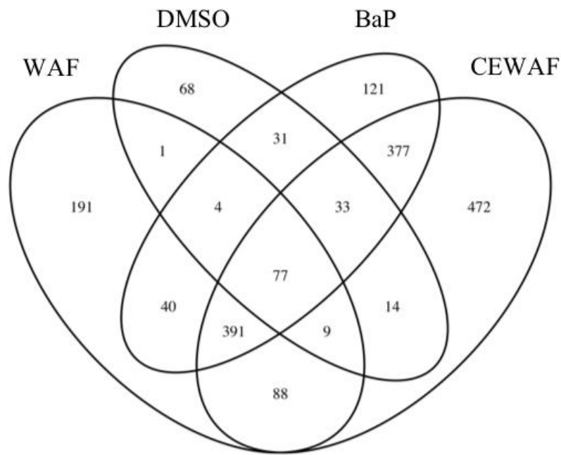
Figure 4: Venn Diagram of the number of differentially expressed genes in each treatment compared to control.
