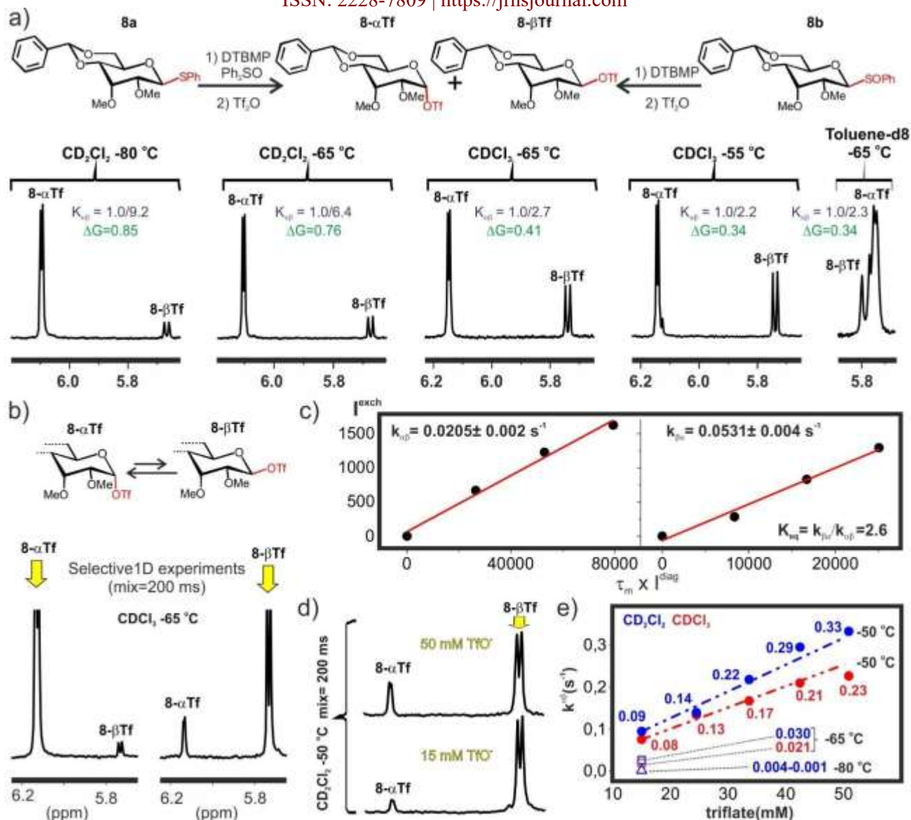
FIGURE 6.- a) Relative equilibrium concentrations for the \alpha - and \beta -allosyl triflates ( 8- \alpha Tf and 8- \beta Tf ) generated from donors 8a or 8b , under different solvent and temperature conditions, as revealed by 1D-NMR. The resulting K_{\alpha/\beta} and \Delta G (Kcal/mol) values are indicated. b) Example of selective NOESY-1D experiments acquired with excitation of either the \alpha or \beta anomeric signals (left and right, respectively). c) EXSY plots. Linear fittings (red lines) provided the rate constants, which were independently determined for the \alpha \rightarrow \beta and \beta \rightarrow \alpha processes (left and right, respectively). d) NOESY-1D experiments acquired with two different concentrations of triflate anion. e) Anomerization rate constants determined under different experimental conditions (solvent, temperature and triflate anion concentration).
