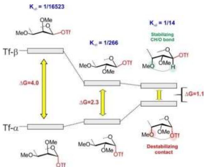
FIGURE 5. -Free energy differences between \alpha - and \beta -glycosyl triflates for D-manno-, D-gluco- and D-allo-derivatives (in the gas phase) computed by quantum mechanics calculations (PCM(CHCl 3 )/M06-2X/6-31G(d,p)level). The predicted K_{\alpha\beta} equilibrium constants are represented in blue.
