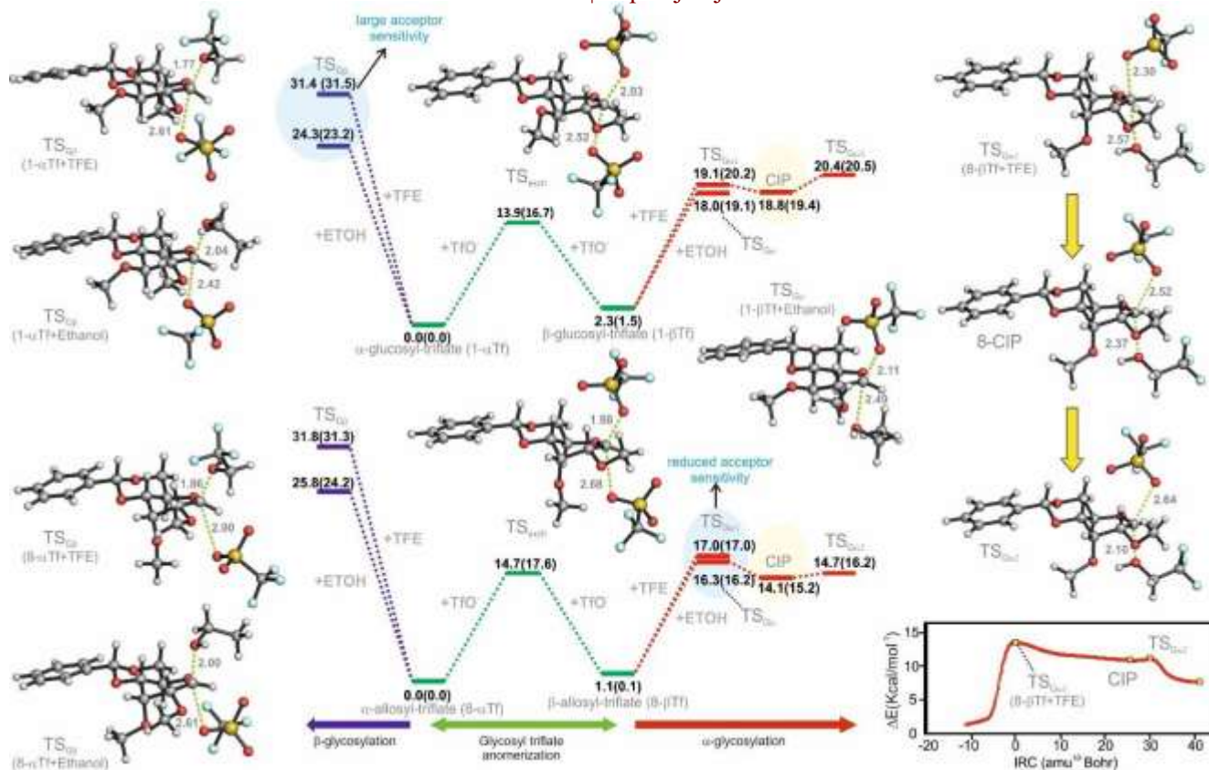
FIGURE 8.- Relative stabilities for the transition states and intermediates involved in the anomeric substitution of glucosyl (up) and allosyl (down) triflates with ethanol and trifluoroethanol (employed notation is shown below), evaluated by quantum mechanics. Computed geometries for selected transition states and intermediates are also represented. The reaction coordinate calculated for the anomeric substitution of the β-allosyl triflate with trifluoroethanol is shown at the bottom-right corner, together with the geometry of the pertaining TSs/intermediates along this path (above). Geometries and intrinsic reaction coordinates (IRC) were calculated with PCM(CHCl 3 )/M06-2X/6-31G(d,p). Relative free energies (ΔG and ΔG ‡ ) are given in kcal/mol and interatomic distances in angstroms. Relative stabilities derived through single-point energy calculations at the SMD(CHCl 3 )/M06-2X/6-311++G(2d,p)/PCM(CHCl 3 )/M06-2X/6-31G(d,p) level are shown in parentheses.
