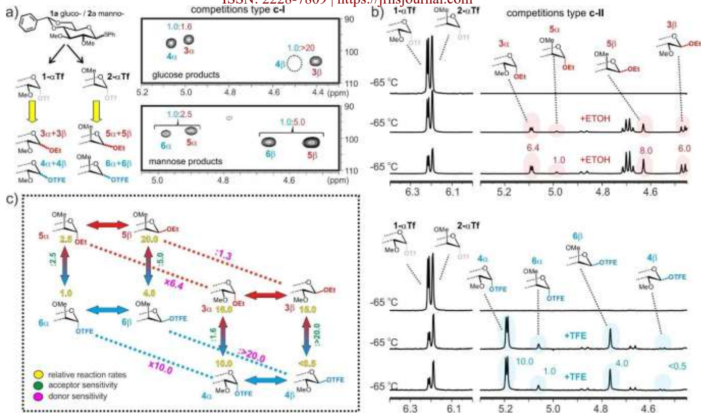
FIGURE 2.- a) Competitions type c-I . The obtained glycoside mixtures were analyzed by means of 1D or 2D-HSQC experiments (anomeric region shown). Relative populations are indicated. b) Competitions type c-II carried out employing ethanol (upper panels) and trifluoroethanol (lower panels) as acceptors. For each alcohol two consecutive sub-stoichiometric additions were performed. Relative populations for the alternative glycoside products are shown. c) Chart showing the combined values obtained from competitions c-I and c-II that allowed estimating the relative formation rates for the eight possible glycosylation products (in yellow), together with the ratios representing the acceptor and donor sensitivities (in green and magenta, respectively).
