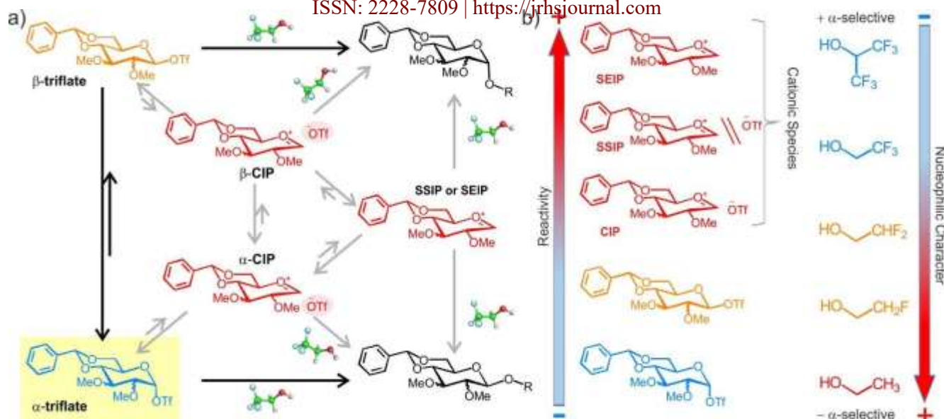
FIGURE 1.- a) Schematic representation of the multiple S_N2/S_N1 reaction pathways leading to the formation of \alpha - and \beta -glycosides from glycosyl triflate intermediates. CIP, SSIP and SEIP stand for contact ion pair, solvent separated ion pair, and solvent equilibrated ion pair, respectively. b) Reactivity gradient for the potential donor intermediates and acceptor alcohols. Glycosylations with weakly nucleophilic alcohols proceed with increased \alpha -stereoselectivity.
