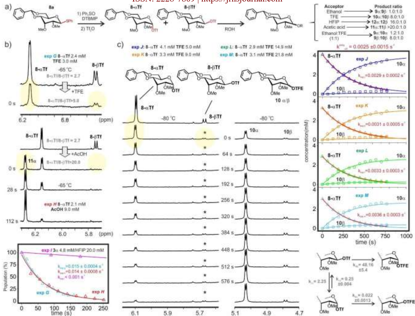
FIGURE 7.- a) Product ratios obtained upon treatment of triflates 8- \alpha Tf + 8- \beta Tf with different acceptors or acceptor mixtures (competitions type c-I , last entry). b) Kinetics experiments G-I (initial 8- \alpha Tf and acceptor concentrations indicated) performed in \text{CDCl}_3 at -65^\circ\text{C} . Selected 1D data sets, before and after addition of the acceptor (TFE or acetic acid), are shown. The anomeric triflate ratios (represented in grey) reveal the preferential consumption of the \beta -stereomer by the acceptor. Reaction curves for the consumption of the major \alpha -allosyl triflate 8- \alpha Tf , together with the corresponding first-order fittings and rate constants derived thereof are shown at the bottom. c) Kinetics experiments J-M performed in \text{CD}_2\text{Cl}_2 at -80^\circ\text{C} (initial 8- \alpha Tf and acceptor concentrations indicated). The time evolution of the allosyl triflate mixture in experiment J as monitored by 1D NMR is displayed on the left. Reaction curves derived from experiments J-M are represented on the right. First-order fittings and rate constants are shown in red. The solid colored lines represent the simultaneous least-squares fitting of the twelve curves to the kinetic model shown at the bottom-right corner. The resulting kinetic constants are represented in grey.
