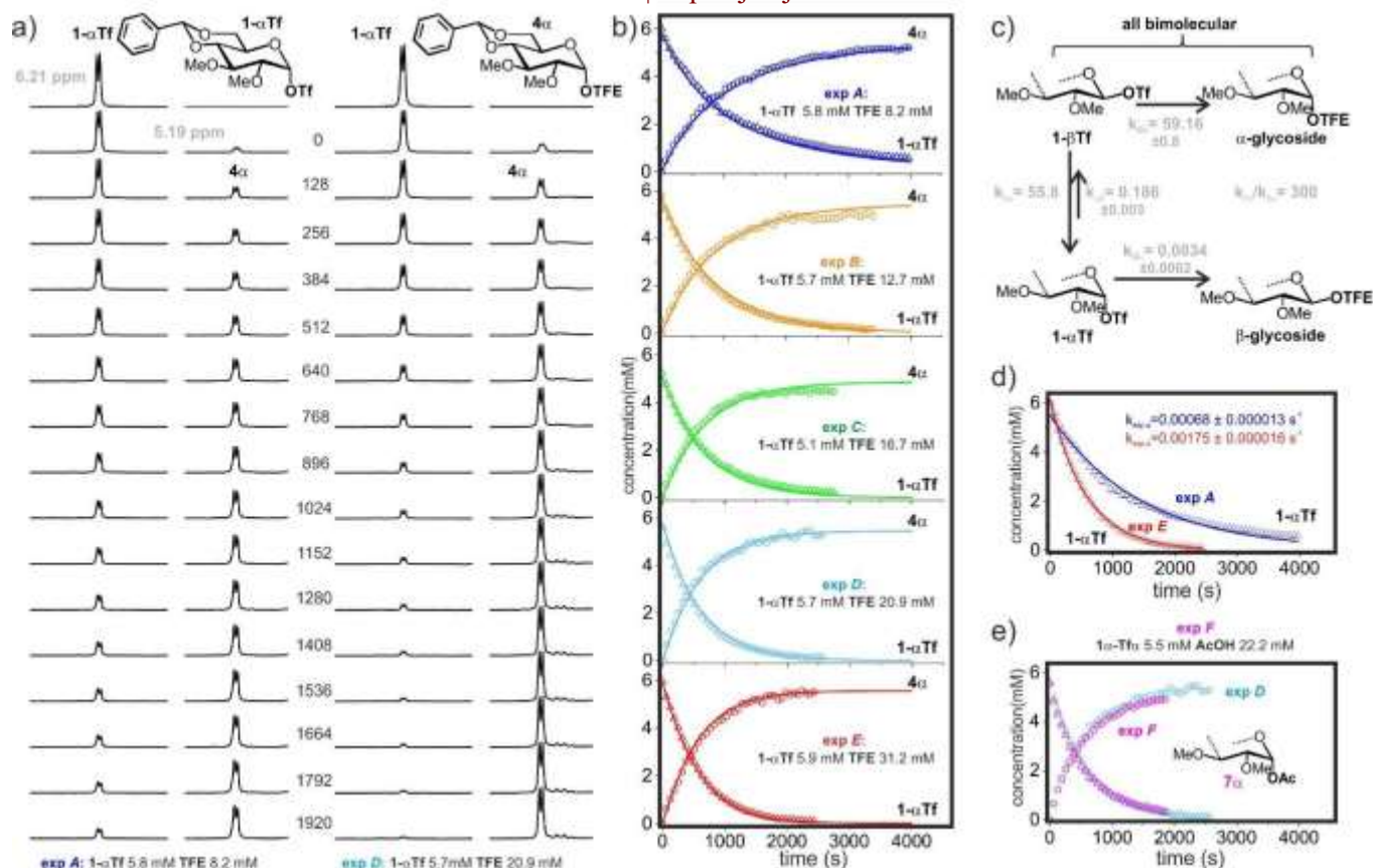
FIGURE 4.- a) Time evolution of 1- \alpha Tf in CDCl 3 at -65 °C upon addition of trifluoroethanol (experiments A and D). b) Experimental reaction curves (circles and triangles) derived from experiments A-E. The solid lines represent the simultaneous least-squares fitting of the ten curves to the kinetic model shown on panel c. c) Kinetic model employed for the analysis of the experimental reaction curves. The resulting kinetic constants are represented in grey. During the fitting procedure the k_{\beta\alpha}/k_{\alpha\beta} ratio was constrained to the experimentally determined range. d) First order fitting of reaction curves for the consumption of 1- \alpha Tf in experiments A and E. e) Experimental curves for experiment D superimposed on that derived from experiment F employing acetic acid as acceptor to yield derivative 7 \alpha .
