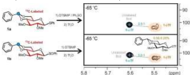
FIGURE 3. - HSQC experiments acquired with triflate mixtures generated upon activation of ^{13}\text{C} -labeled donors 1a and 1b . Cross-peaks corresponding to the (unlabeled) benzyldene CH fragment in the major \alpha -glucosyl triflate intermediate (in cyan), and the ^{13}\text{C} -labeled anomeric CH group in the corresponding \beta -glucosyl triflate (in orange) are shown. Peak relative ratios, together with the estimated population for the \beta -derivative are indicated.
