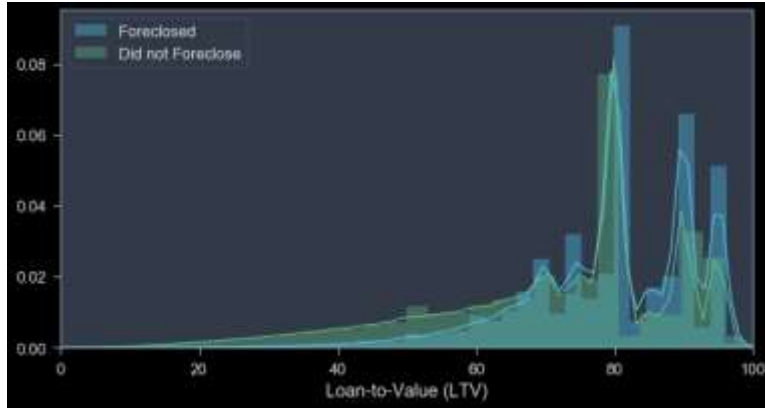
Loan-to-Value
