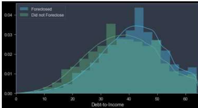
Debt-to-Income
