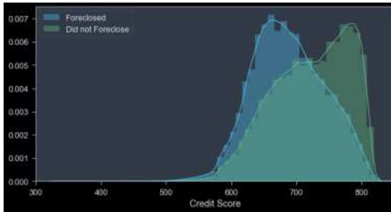
Credit Score
